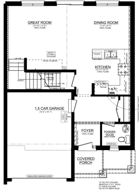
ELMWOOD 'B' UNIT #2 MAINFLOOR PLAN 8' CEILING ON MAIN FLOOR 1.5 CAR 745 SQ. FT.
