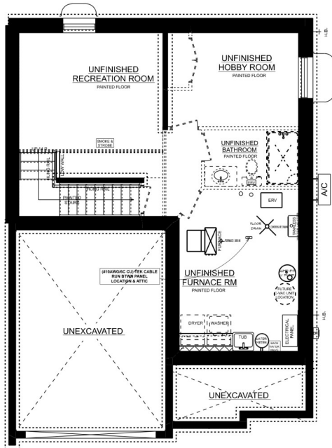
ELMWOOD 'B' UNIT #2 BASEMENT PLAN
