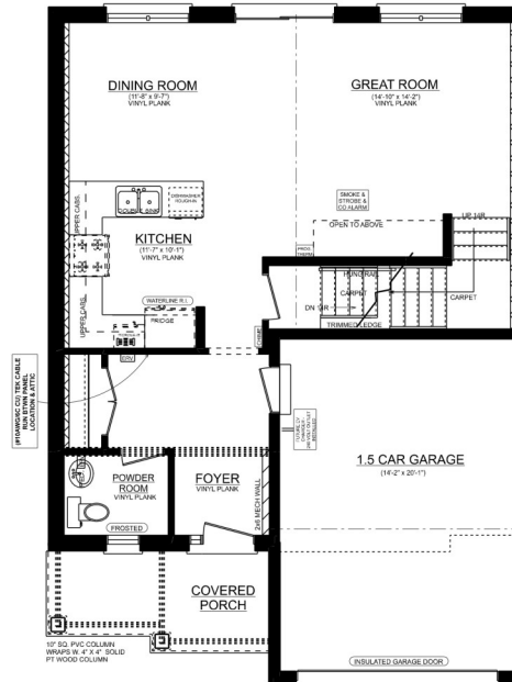
ELMWOOD 'B' UNIT #1 MAINFLOOR PLAN 8' CEILING ON MAIN FLOOR 1.5 CAR 745 SQ. FT.
