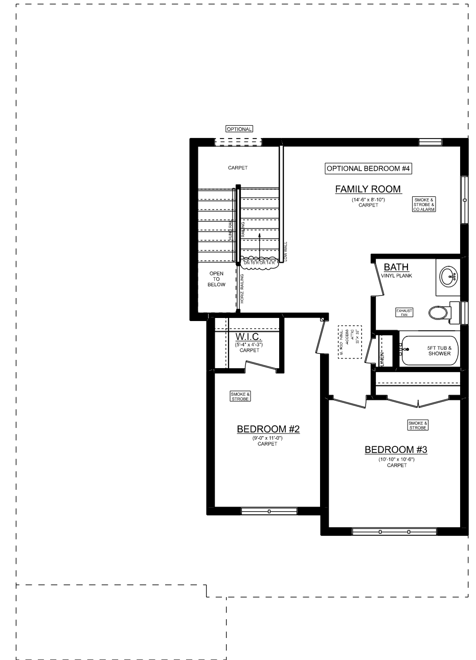
THE STONEHAVEN 'A' 2ND FLOOR PLAN 618 SQ. FT.
