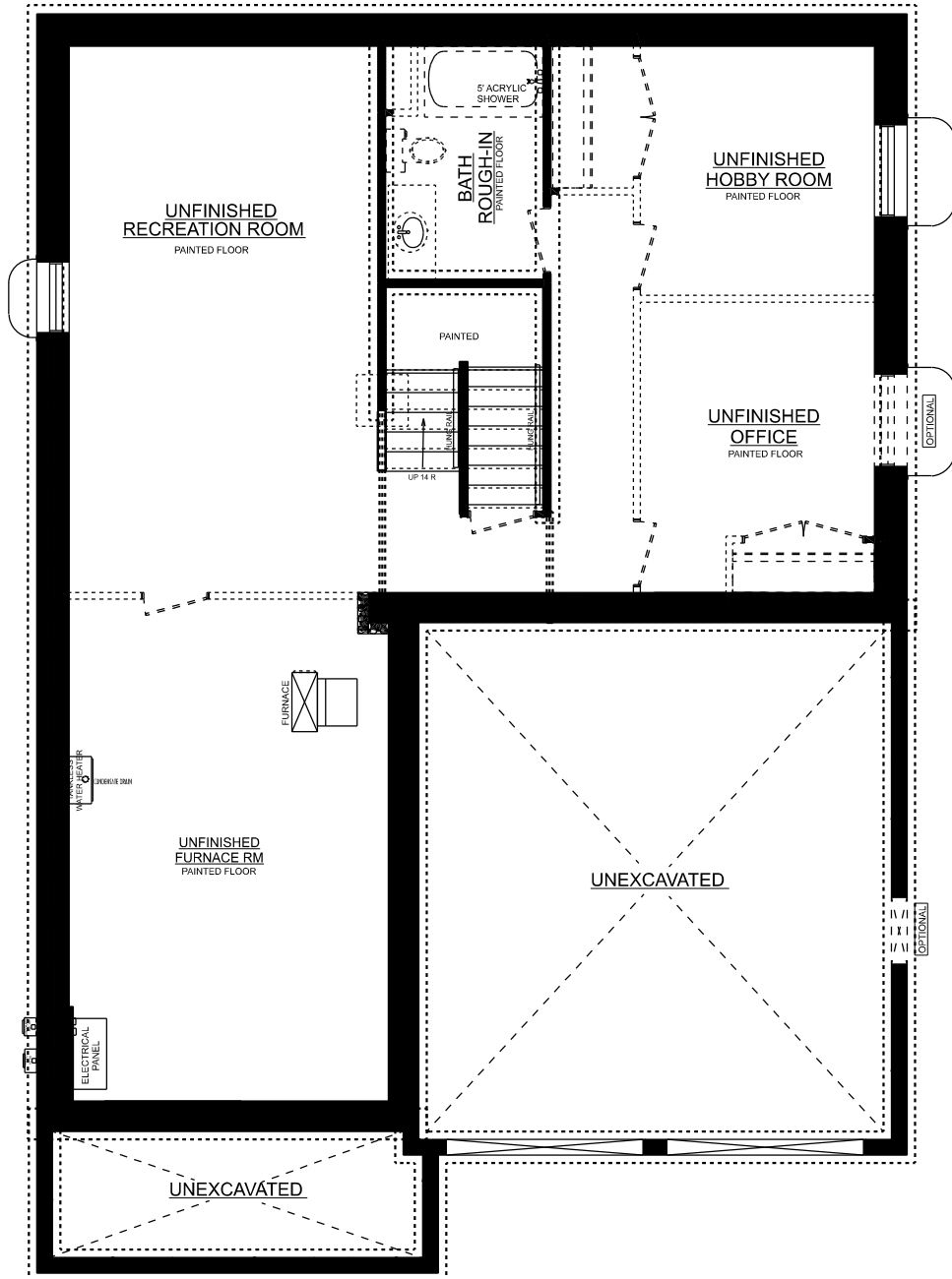
BASEMENT PLAN
