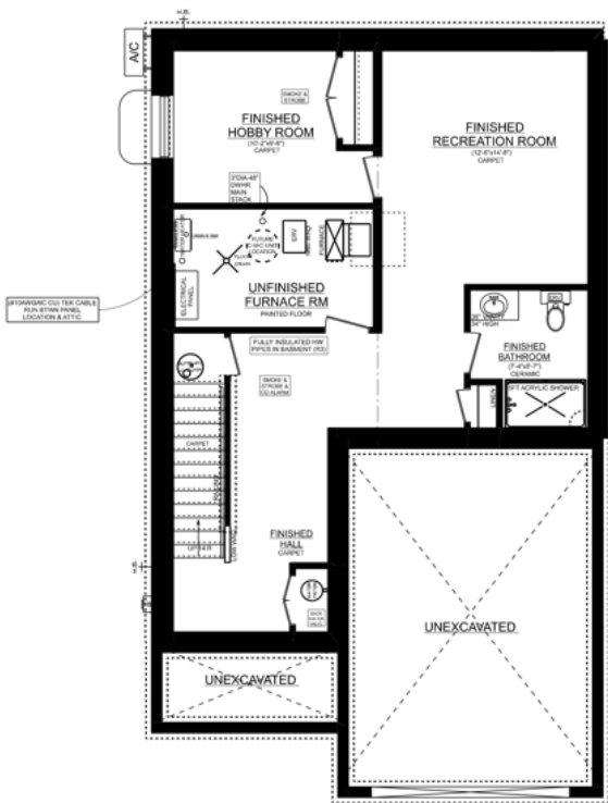
SEDONA 'B' UNIT #1 BASEMENT PLAN 561 SQ. FT. FINISHED BASEMENT AREA
