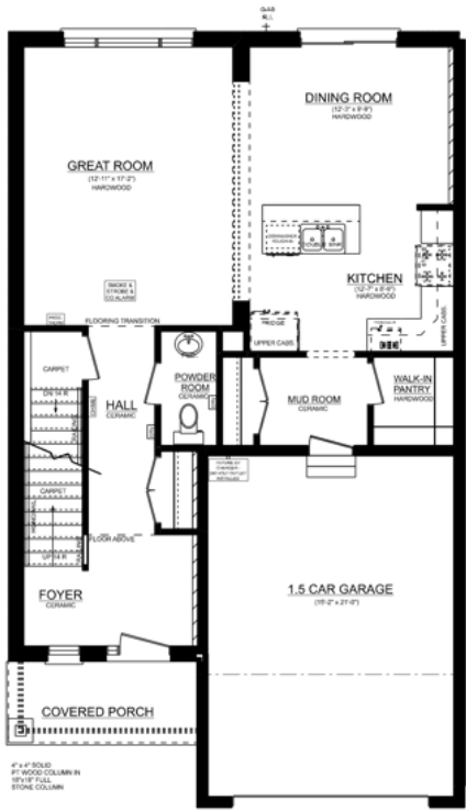
SEDONA 'B' UNIT #1 MAINFLOOR PLAN 8' CEILING ON MAIN FLOOR 1.5 CAR 879 SQ. FT.
