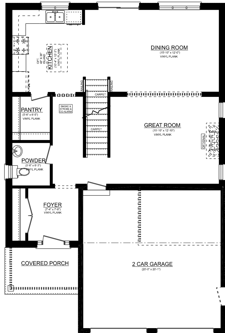
MAIN FLOOR
