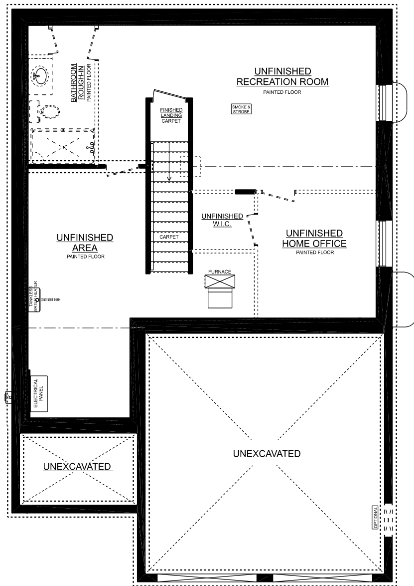
BASEMENT PLAN
