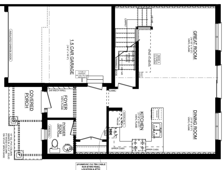
ELMWOOD 'B' UNIT #2 MAINFLOOR PLAN 8' CEILING ON MAIN FLOOR 1.5 CAR 745 SQ. FT.
