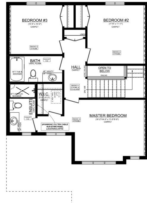
ELMWOOD 'B' UNIT #1 2ND FLOOR PLAN 8' CEILINGS ON 2ND FLOOR 775 SQ. FT. DOES NOT INCLUDE 75 SQ.FT OPEN TO BELOW
