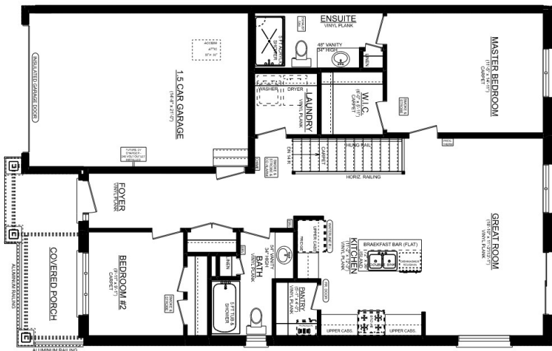
EASTON 'A' UNIT #2 MAIN FLOOR PLAN 1200 SQ. FT. 8\"/>
