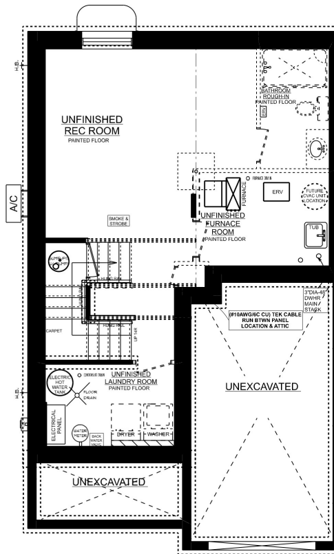
KENSINGTON 'A' UNIT #1 BASEMENT PLAN
