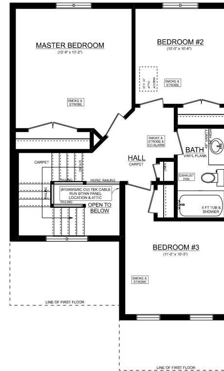
KENSINGTON 'A' UNIT #1 2ND FLOOR PLAN 8' CEILINGS ON 2ND FLOOR 640 SQ. FT. (DOES NOT INCLUDE 90 SQ.FT. OPEN TO BELOW)
