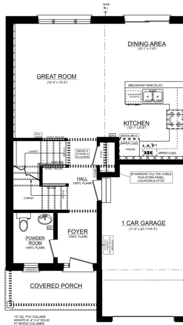
KENSINGTON 'A' UNIT #1 MAINFLOOR PLAN 8' CEILINGS ON MAIN FLOOR 650 SQ. FT. 1 CAR
