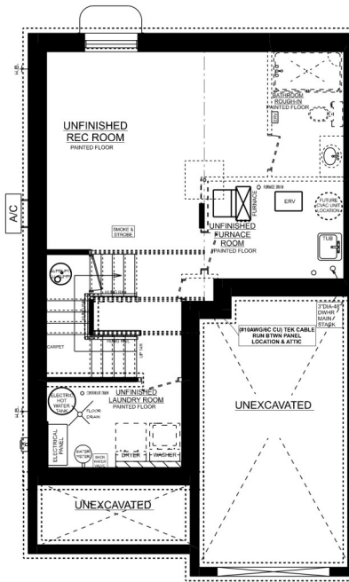
KENSINGTON 'A' UNIT #1 BASEMENT PLAN
