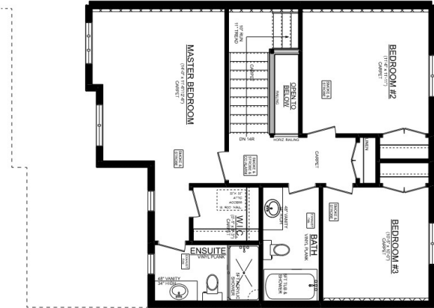
ELMWOOD 'A' UNIT #2 2ND FLOOR PLAN 8' CEILINGS ON 2ND FLOOR 775 SQ. FT.
