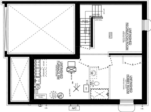
ELMWOOD 'A' UNIT #2 UNFINISHED BASEMENT PLAN
