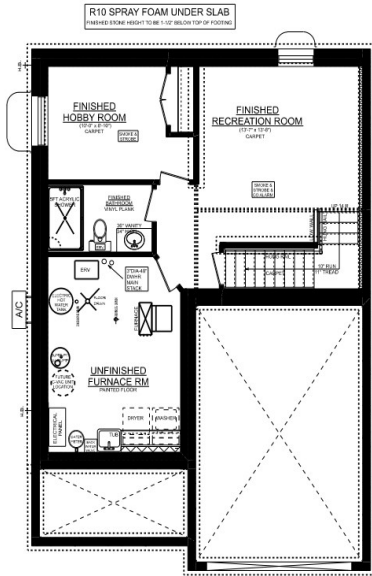
ELMWOOD 'C' UNIT #1 BASEMENT PLAN 433 SQ.FT FINISHED BASEMENT SPACE
