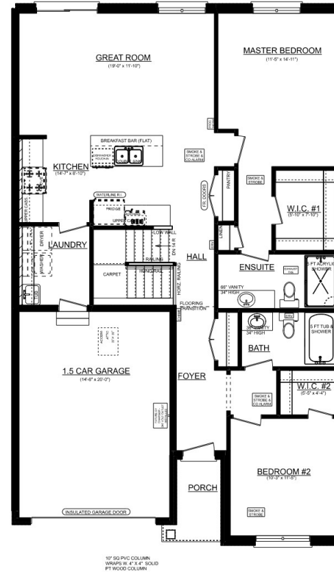
SUTHERLAND 'A' UNIT #2 MAIN FLOOR PLAN 1300 SQ. FT. 8' CEILINGS ON MAINFLOOR
