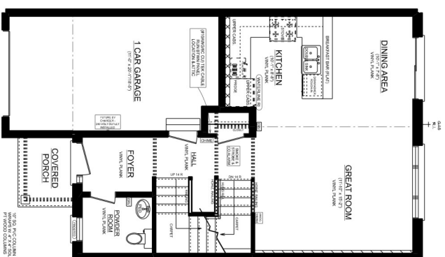
KENSINGTON 'C' UNIT #2 MAIN FLOOR PLAN 8' CEILINGS ON MAIN FLOOR 1 CAR 650 SQ. FT.
