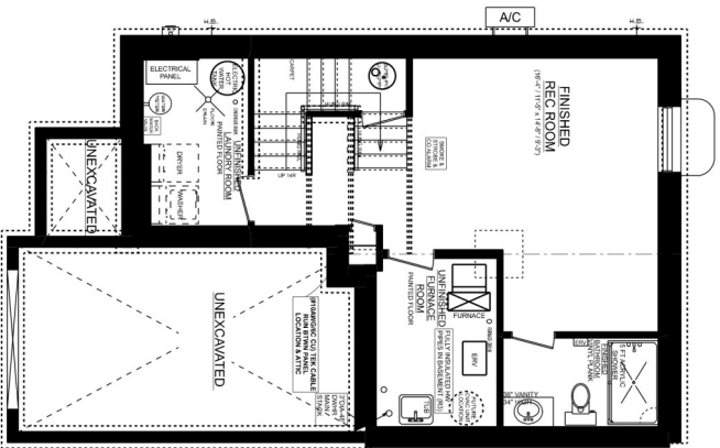
KENSINGTON 'C' UNIT #1 BASEMENT PLAN 310 SQ. FT. FINISHED SPACE
