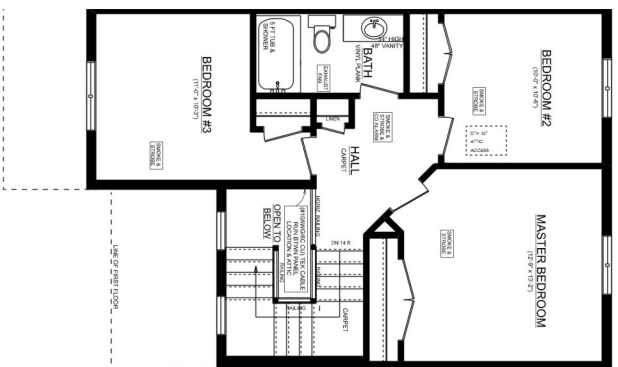
KENSINGTON 'A' UNIT #2 2ND FLOOR PLAN 8 CEILINGS ON 2ND FLOOR 640 SQ. FT. (DOES NOT INCLUDE 90 SQ.FT. OPEN TO BELOW)
