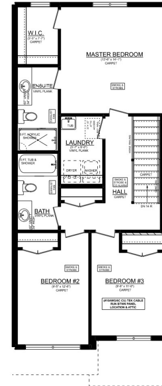
ASHTON 'A' END UNIT #6 2ND FLOOR PLAN 8" CEILINGS ON 2ND FLOOR 910 SQ. FT.
