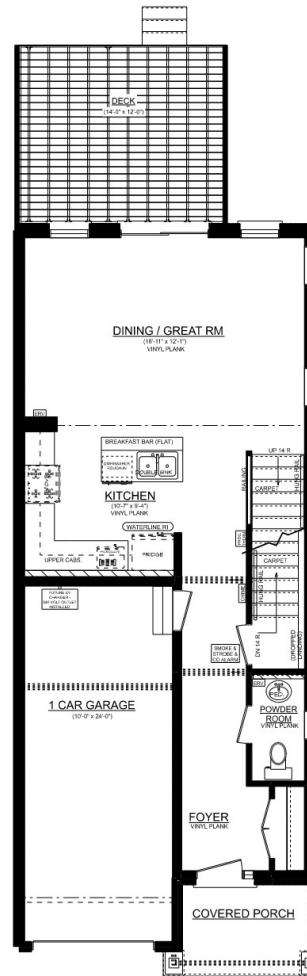
ASHTON 'A' END UNIT #6 MAINFLOOR PLAN 8" CEILINGS ON MAIN FLOOR 690 SQ. FT.
