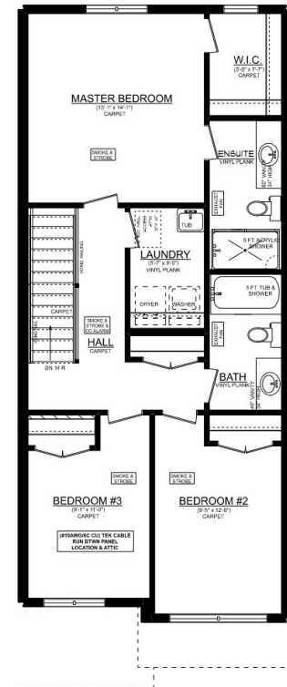
ASHTON 'A' INTERIOR UNIT #5 2ND FLOOR PLAN 8' CEILINGS ON 2ND FLOOR 880 SQ. FT.
