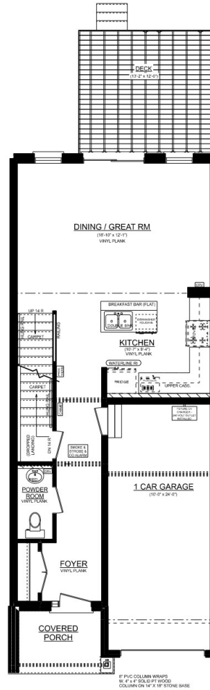
ASHTON 'A' INTERIOR UNIT #5 MAINFLOOR PLAN 8' CEILINGS ON MAIN FLOOR 660 SQ. FT.
