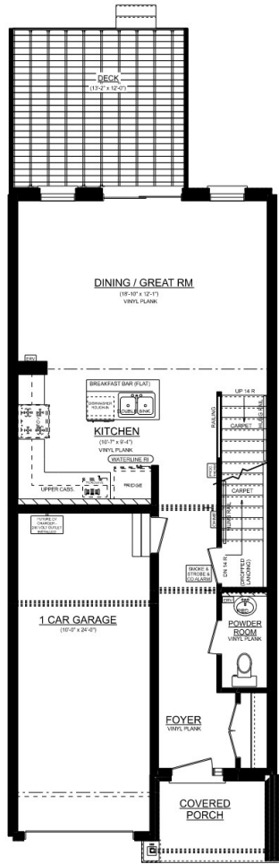
ASHTON 'A' INTERIOR UNIT #4 MAINFLOOR PLAN 8' CEILINGS ON MAIN FLOOR 660 SQ. FT.
