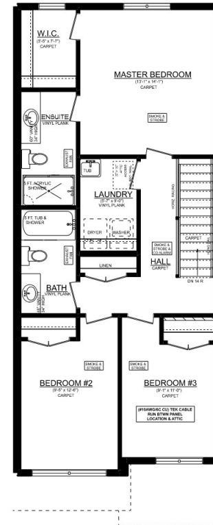
ASHTON 'A' INTERIOR UNIT #2 2ND FLOOR PLAN 8' CEILINGS ON 2ND FLOOR 880 SQ. FT.
