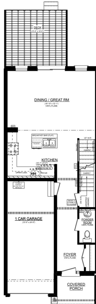
ASHTON 'A' INTERIOR UNIT #2 MAIN FLOOR PLAN 8' CEILINGS ON MAIN FLOOR 660 SQ. FT.
