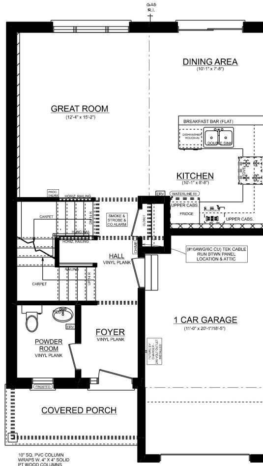
KENSINGTON MAINFLOOR PLAN 8' CEILINGS ON MAIN FLOOR 650 SQ. FT. 1 CAR
