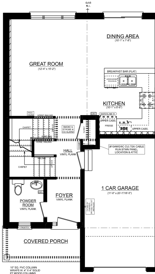
KENSINGTON MAINFLOOR PLAN
