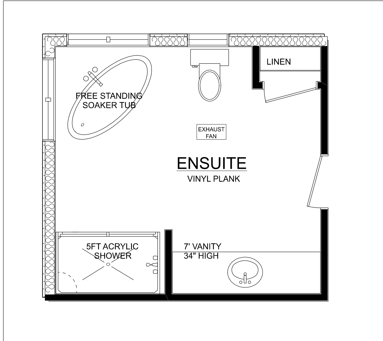
IVYSTONE OPTIONAL DELUXE ENSUITE #1 to Deluxe Ensuite design includes 5ft acrylic shower, oval freestanding tub w/ floor taps, 7 ft vanity w. 1 sink. Relocate 48"x36" window to above tub on rear, add a 48"x36" csmt to side elevation above tub and a 24"x36" csmt to rear above toilet. Include a Linen closet (includes relocated smaller WIC).
