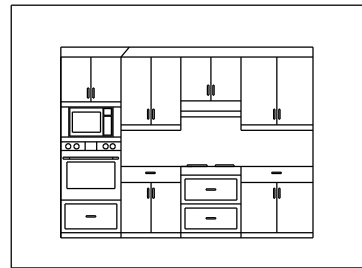
DUNMOOR KITCHEN w. WALL OVEN ELEVATION w. STANDARD RANGE HOOD
