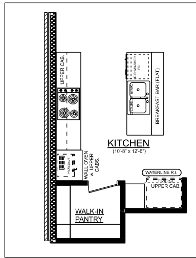
DUNMOOR OPTIONAL KITCHEN LAYOUT w. WALL OVEN
