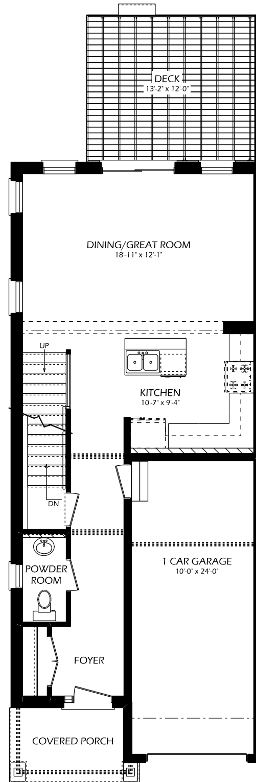
MAIN FLOOR 690 SQ. FT. 8' CEILINGS ON MAIN FLOOR
