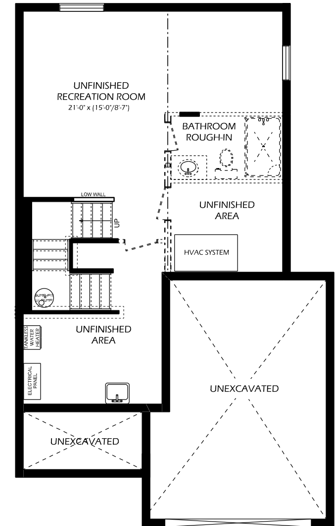
BASEMENT
