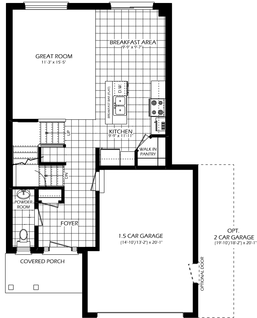
MAIN FLOOR 700 SQ. FT. 8' CEILINGS (ON MAIN FLOOR)
