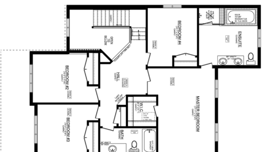
EDENBROOK 'A' 2ND FLOOR PLAN 1212 SQ. FT. (DOES NOT INCLUDE 82 SQ. FT. OPEN TO BELOW) 8' CEILINGS ON 2ND FLOOR
