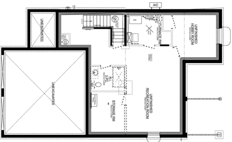
EDENBROOK 'A' BASEMENT PLAN
