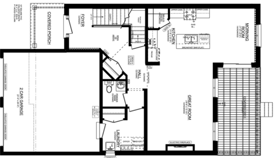
EDENBROOK 'A' MAIN FLOOR PLAN 980 SQ. FT. 8' CEILINGS ON MAIN FLOOR
