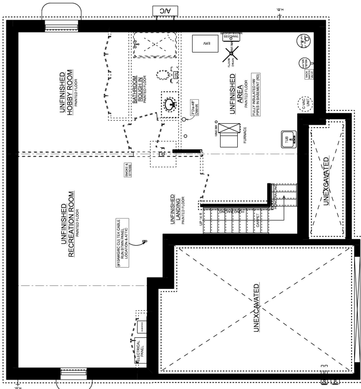
THE KNOLLWOOD 'A' BASEMENT PLAN
