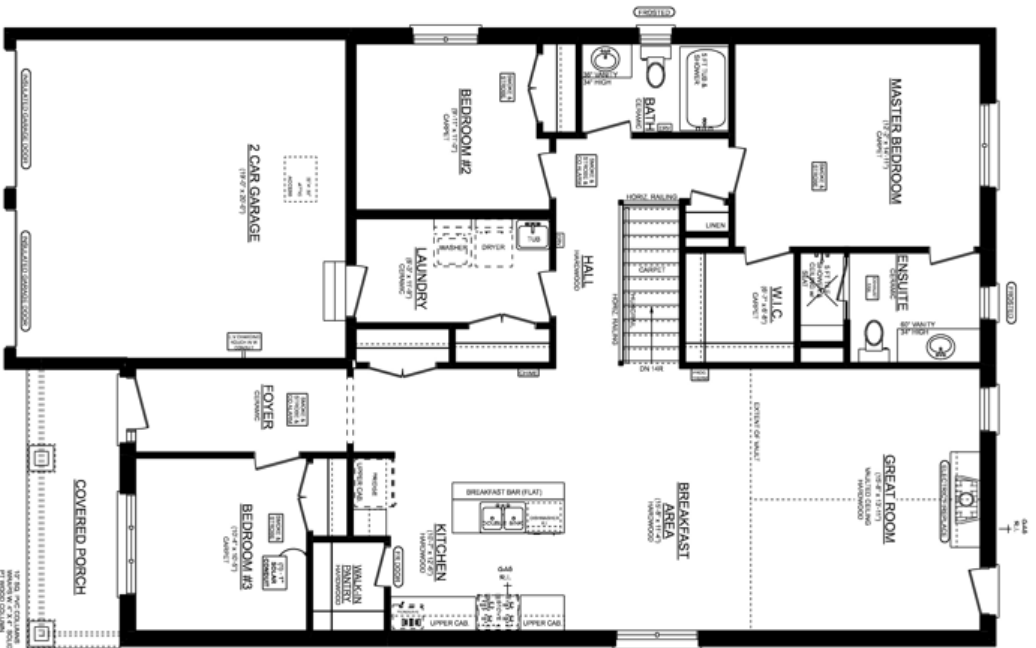
DUNMOOR 'B' MAIN FLOOR PLAN 1884 SQ. FT. & CEILINGS ON MAIN FLOOR
