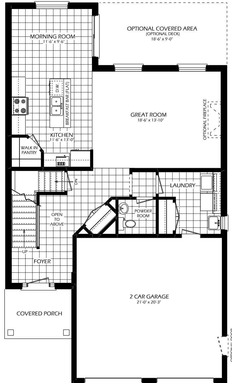
MAIN FLOOR 980 SQ. FT.
