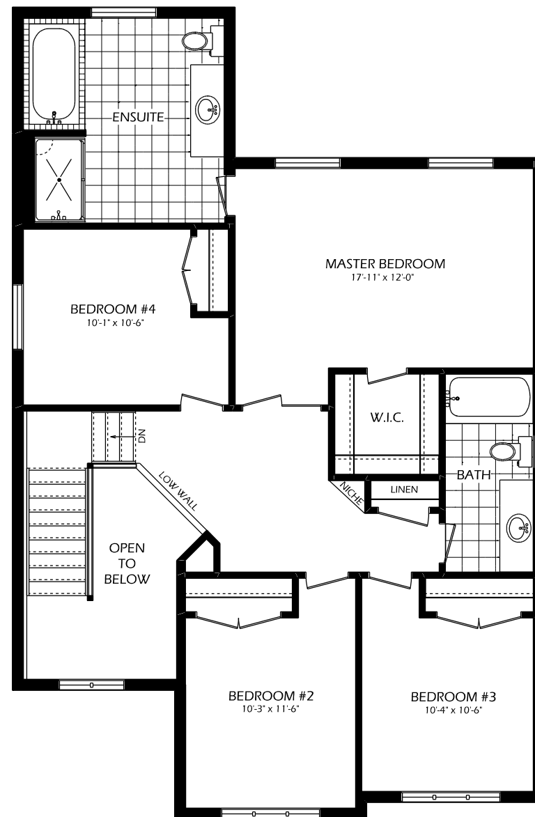
2ND FLOOR 1160 SQ. FT. 134 SQ. FT. OPEN TO BELOW
