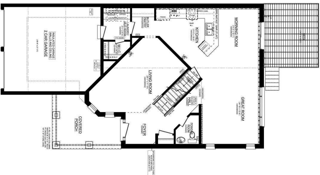
WINDFLOWER 'B' MAINFLOOR PLAN
