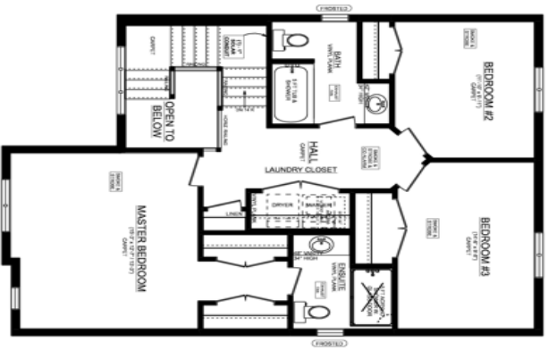
MAPLERIDGE 'A' 2ND FLOOR PLAN 924 SQ. FT. (DOES NOT INCLUDE 42 SQ. FT. OPEN TO BELOW) & CEILINGS ON 2ND FLOOR
