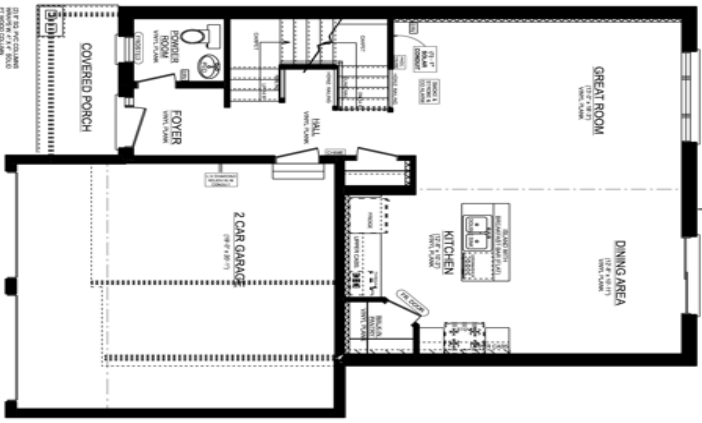
MAPLERIDGE 'A' MAIN FLOOR PLAN 797 SQ. FT. 2 CAR & CEILINGS ON MAIN FLOOR
