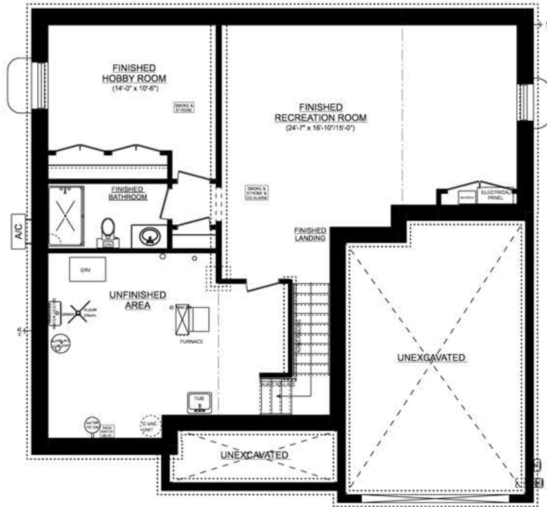
THE KNOLLWOOD 'A' BASEMENT PLAN 687 SQ.FT. FINISHED BASEMENT SPACE
