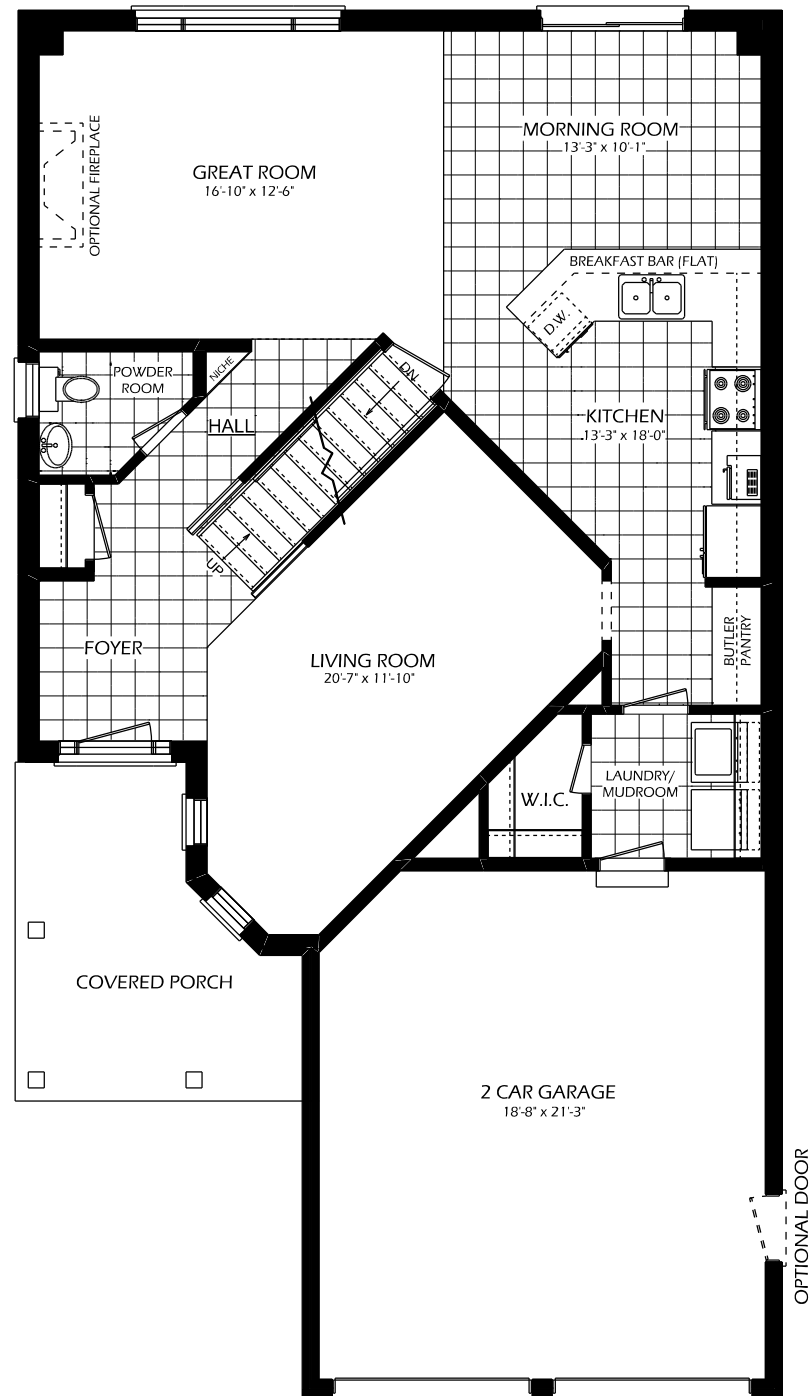
MAIN FLOOR 1127 SQ. FT. 8' CEILING (MAIN FLOOR)
