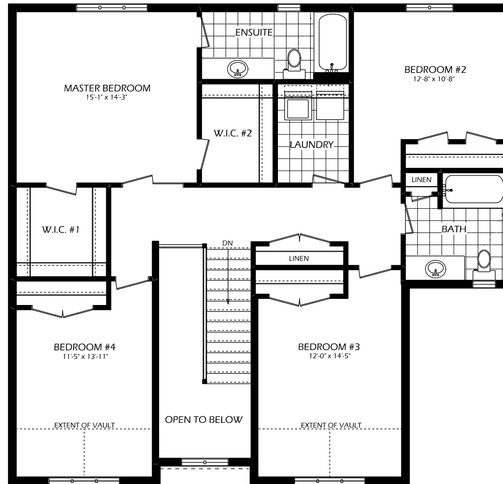
2ND FLOOR 1378 SQ.FT. 8' CEILINGS (2ND FLOOR)
