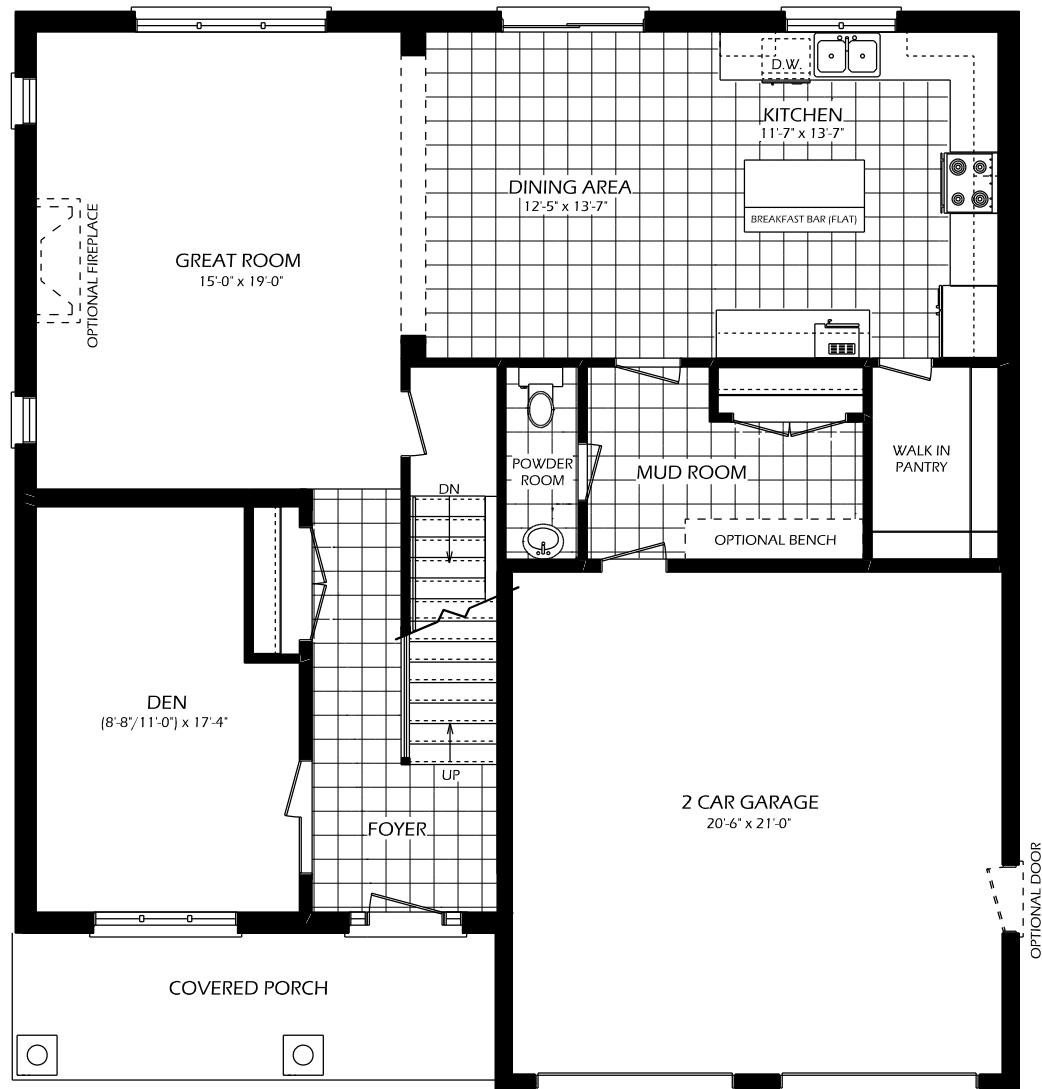
MAIN FLOOR 1288 SQ.FT. 8' CEILINGS (MAIN FLOOR)
