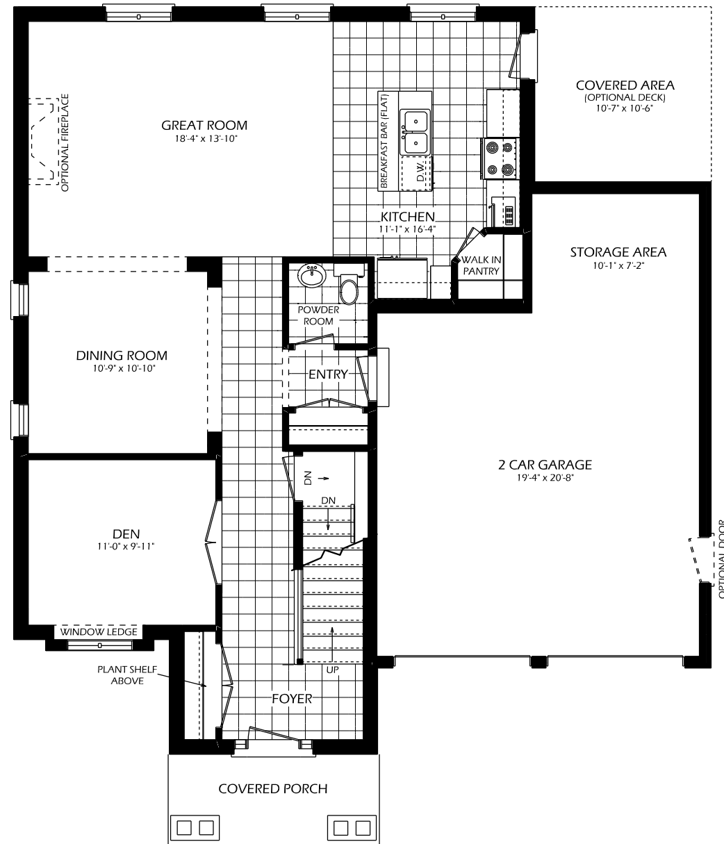
MAIN FLOOR 1084 SQ. FT. 8' CEILINGS (ON MAIN FLOOR)
