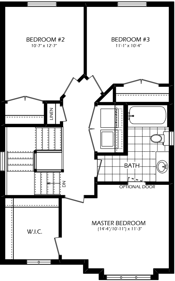
2ND FLOOR 830 SQ. FT. 8' CEILINGS (ON 2ND FLOOR)
