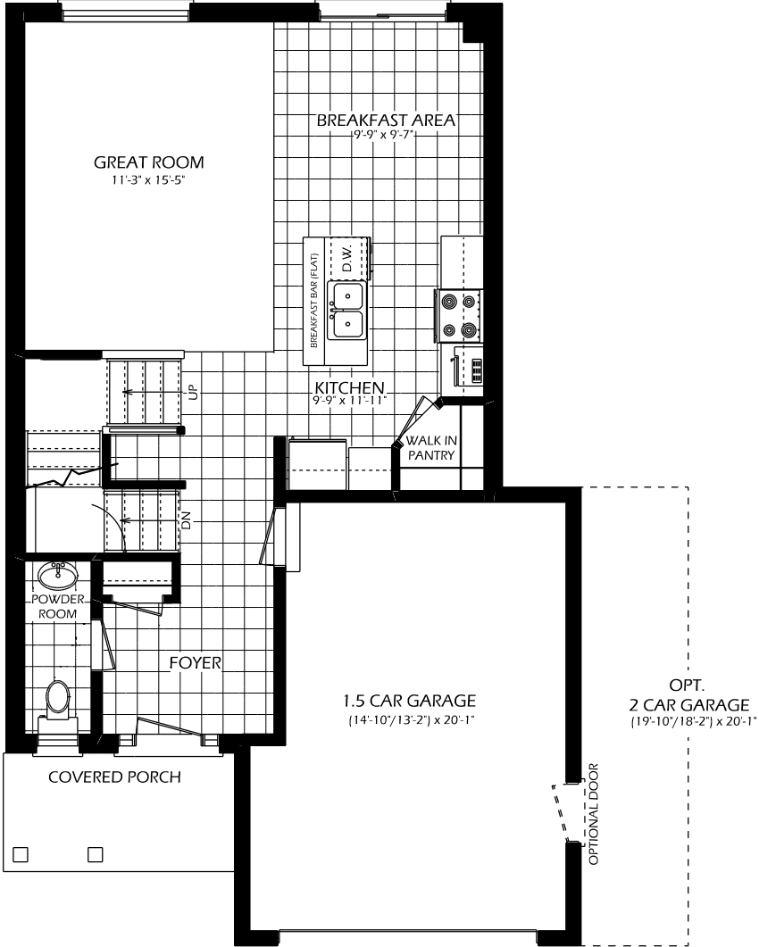
MAIN FLOOR 698 SQ. FT. 8' CEILINGS (ON MAIN FLOOR)
