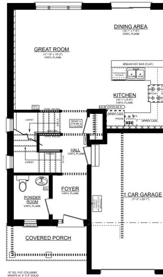
KENSINGTON 'B' UNIT #1 MAIN FLOOR PLAN 8' CEILINGS ON MAIN FLOOR 650 SQ. FT.
