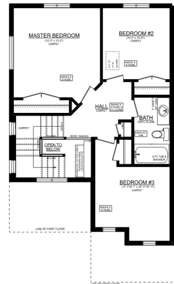
KENSINGTON 'B' UNIT #1 2ND FLOOR PLAN 8' CEILINGS ON 2ND FLOOR 640 SQ. FT.
