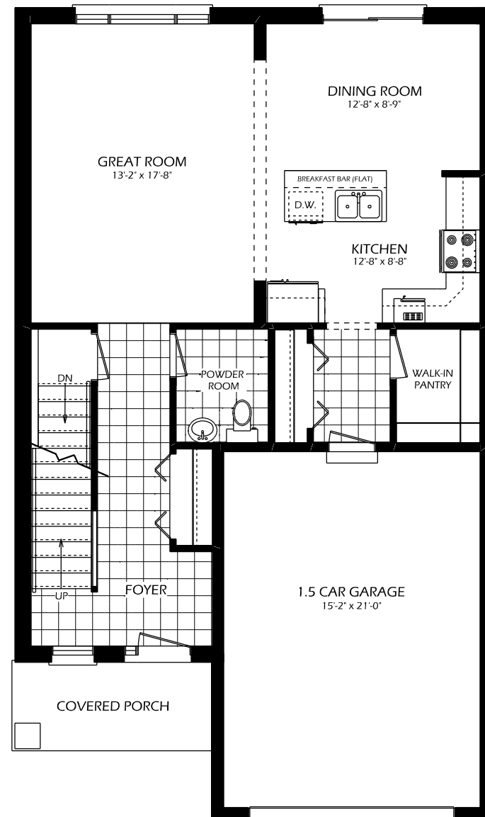
MAIN FLOOR 878 SQ. FT. 8' CEILING ON MAIN FLOOR
