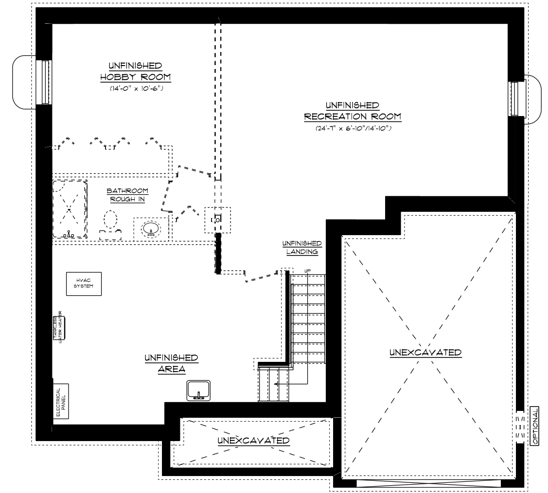
THE KNOLLWOOD BASEMENT PLAN
