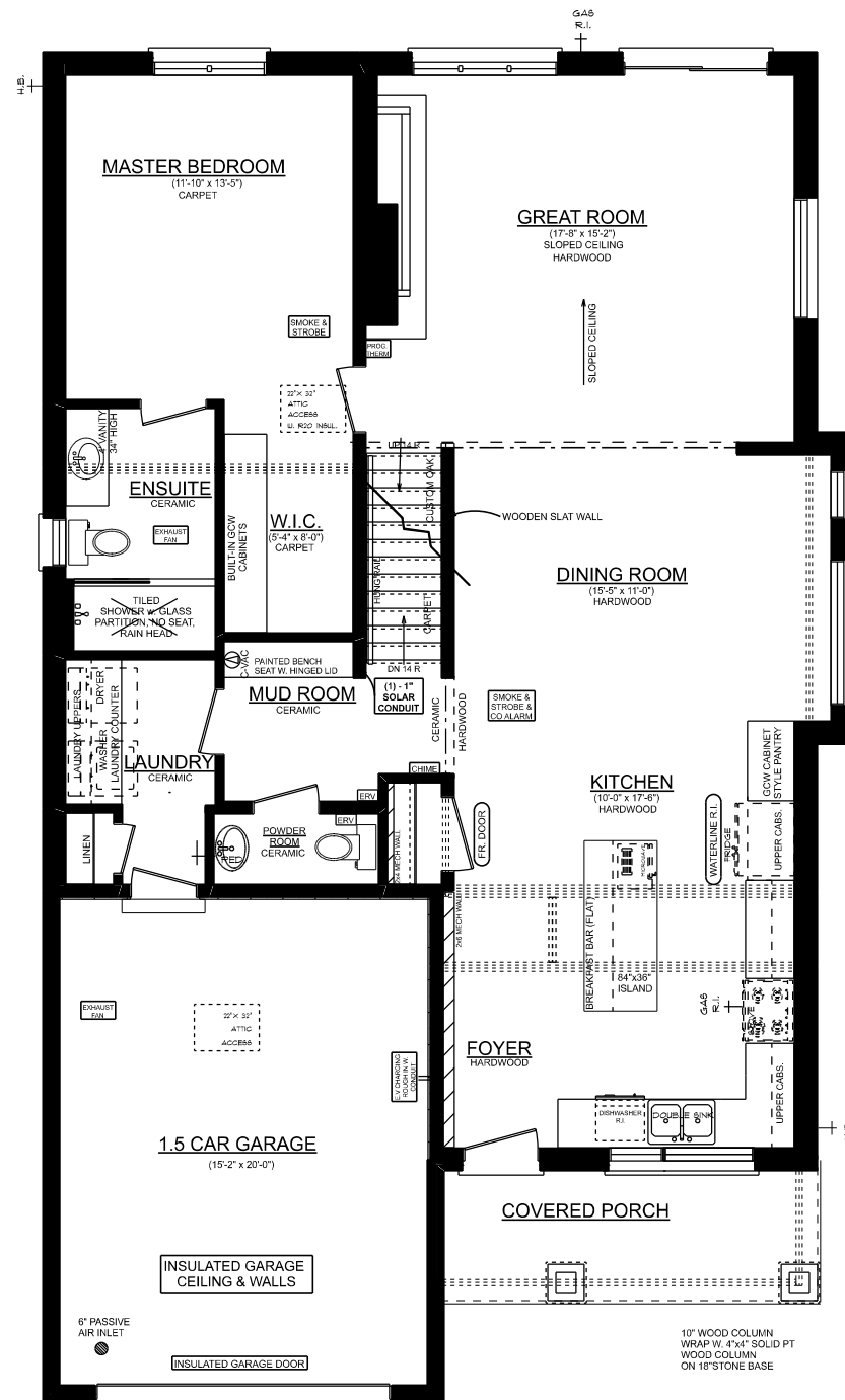
PALMER 'A' MAIN FLOOR 1307 SQ.FT. 8' CEILINGS ON MAINFLOOR
