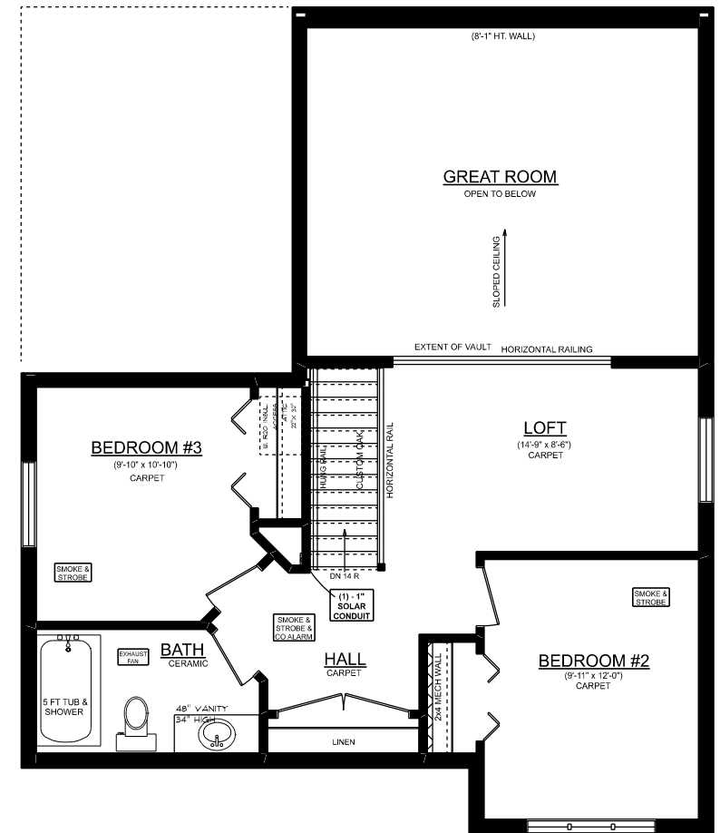
PALMER 'A' 2ND FLOOR 627 SQ.FT. 8' CEILINGS ON MAINFLOOR
