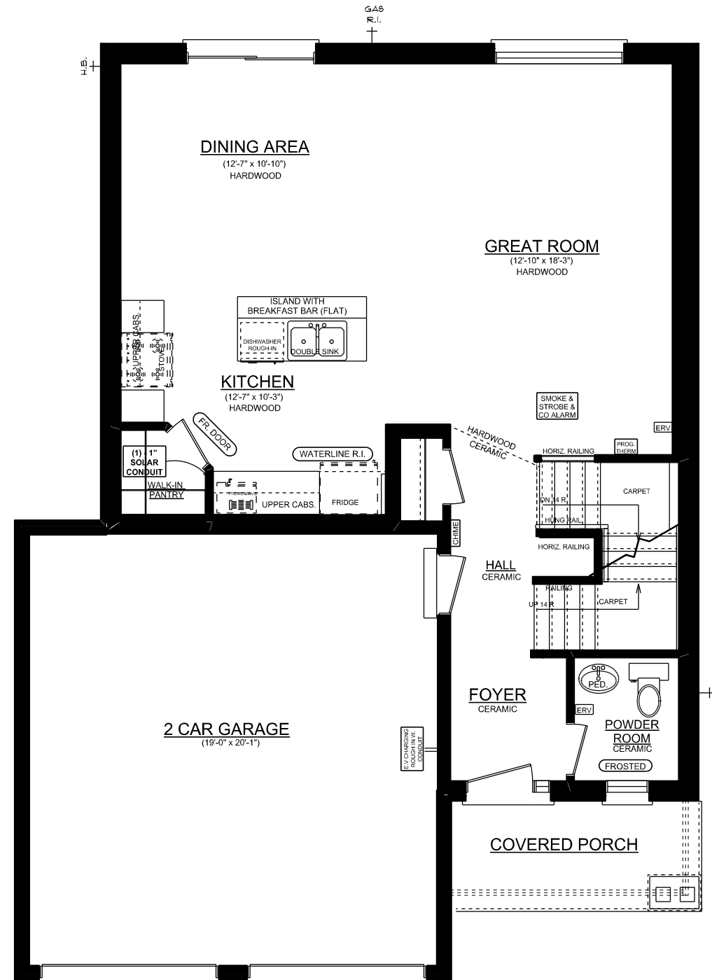
MAPLERIDGE 'A' MAINFLOOR PLAN 785 SQ. FT. 2 CAR 8' CEILINGS ON MAINFLOOR
