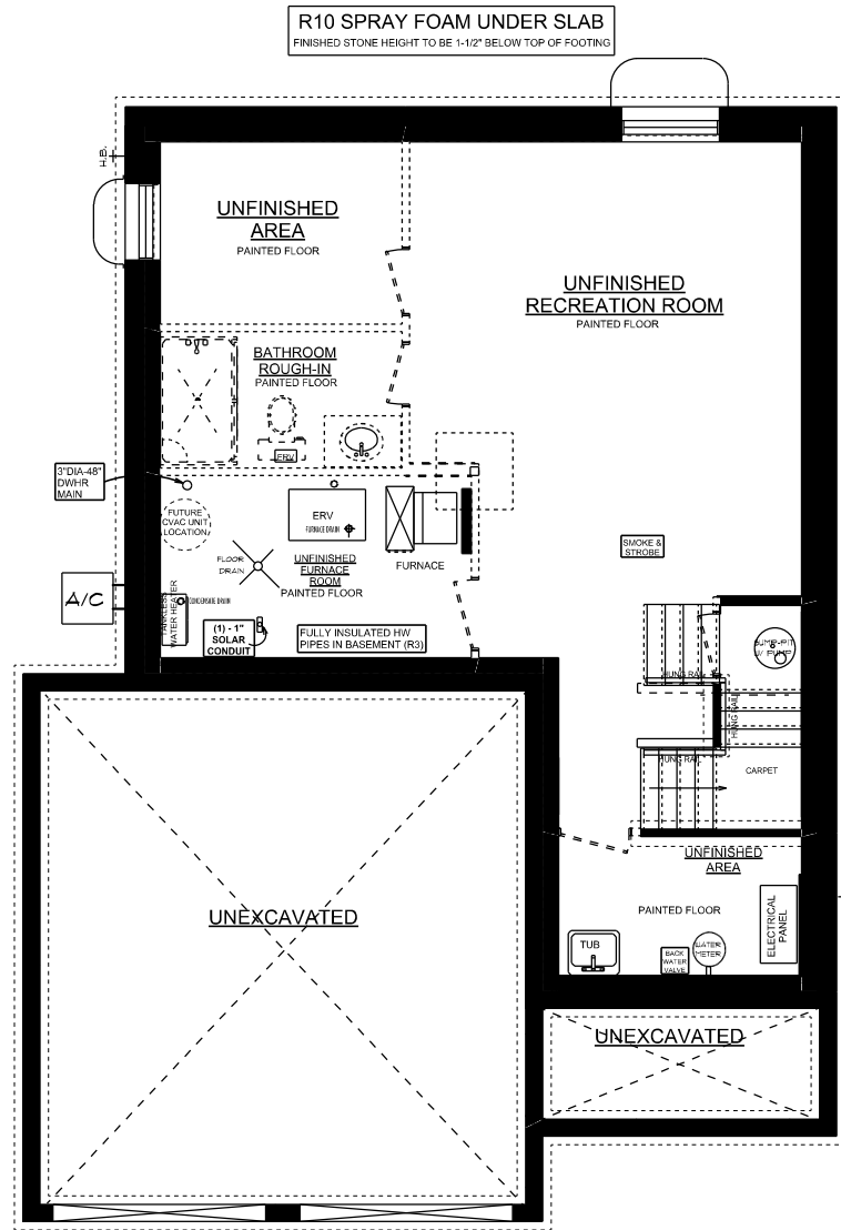
MAPLERIDGE 'A' BASEMENT PLAN
