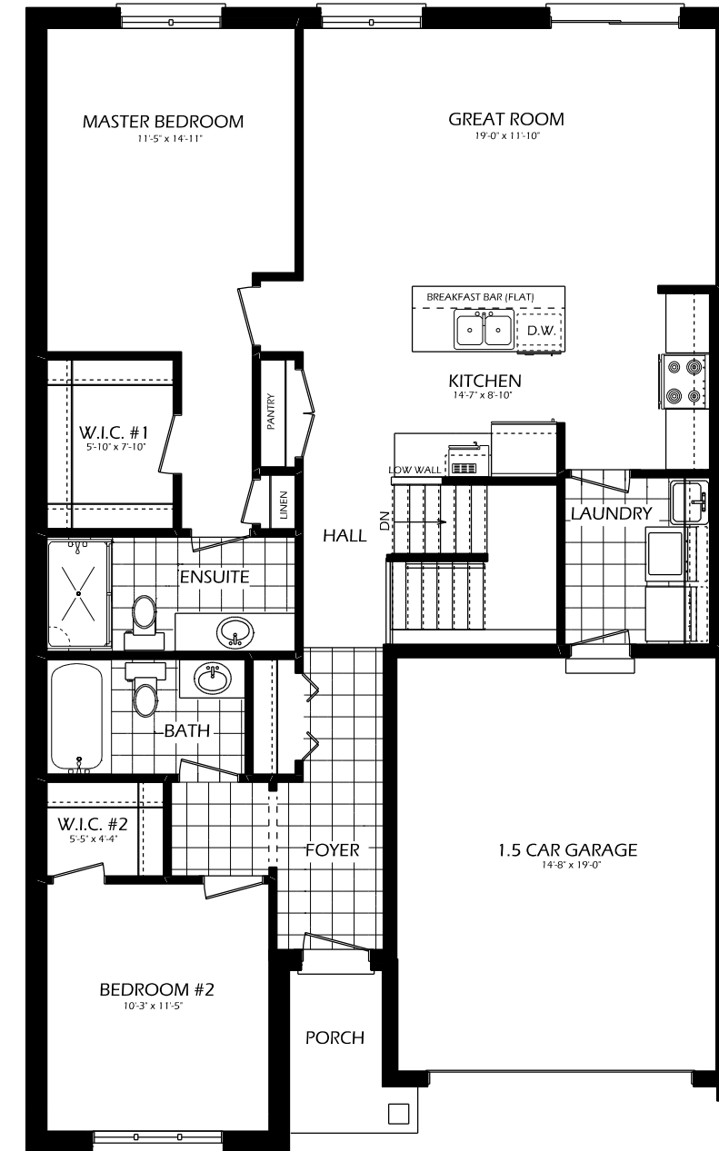
MAIN FLOOR 1300 SQ. FT. 8' CEILINGS ON MAINFLOOR
