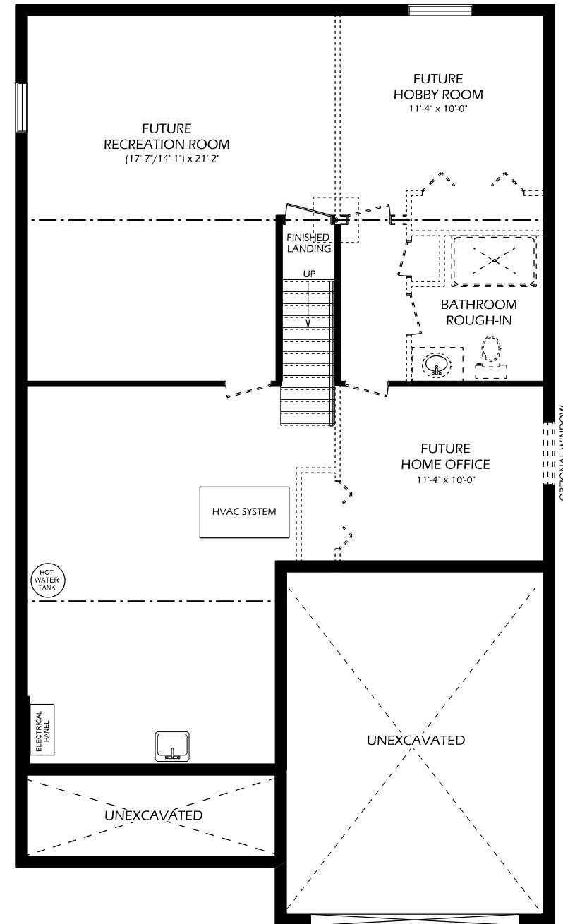
BASEMENT
