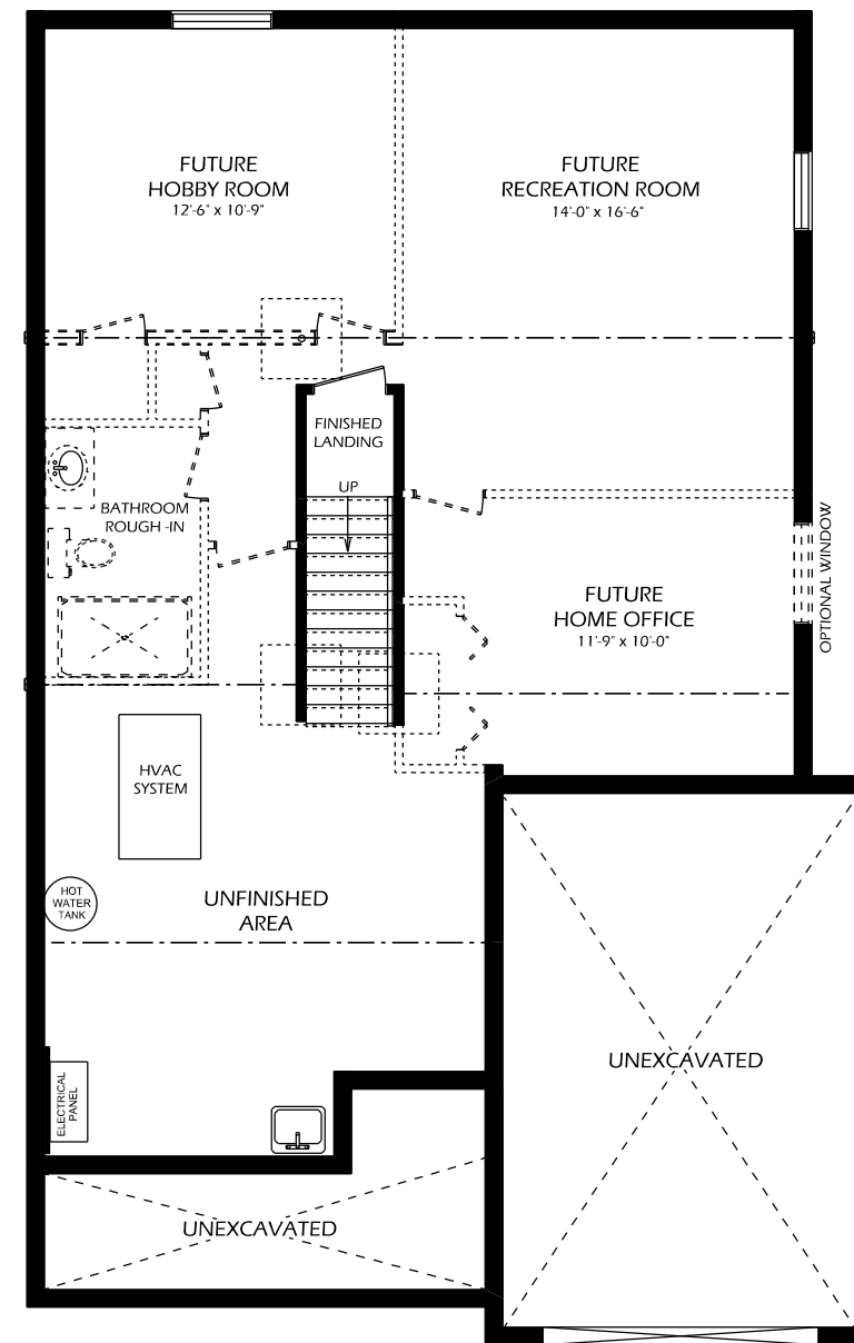
BASEMENT
