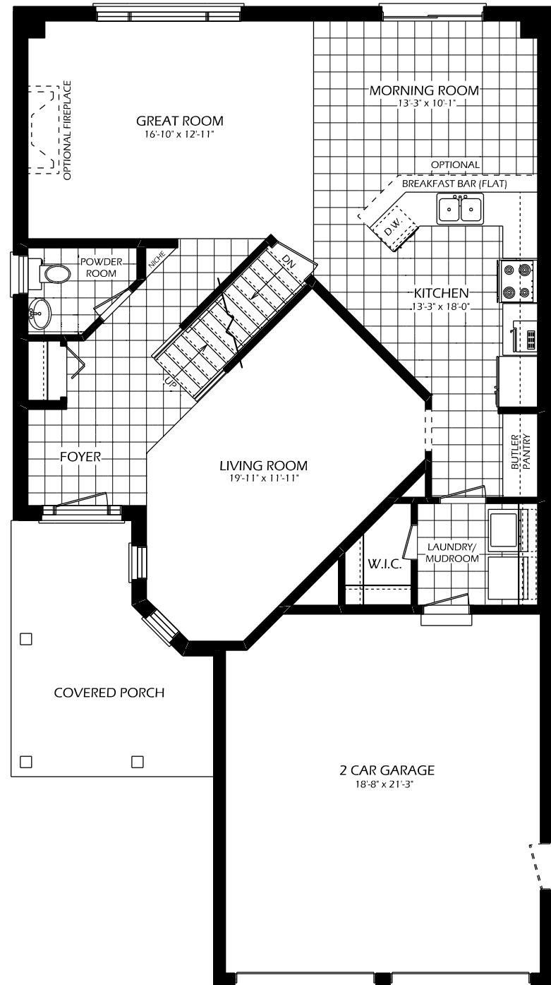
MAIN FLOOR 1118 SQ. FT. 8' CEILING (MAIN FLOOR)
