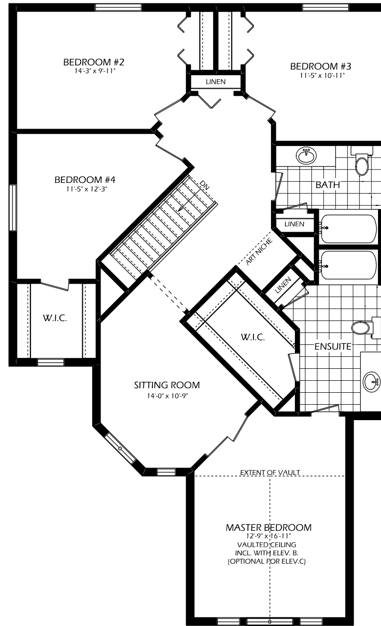
2ND FLOOR 1346 SQ. FT. 8' CEILINGS (2ND FLOOR)
