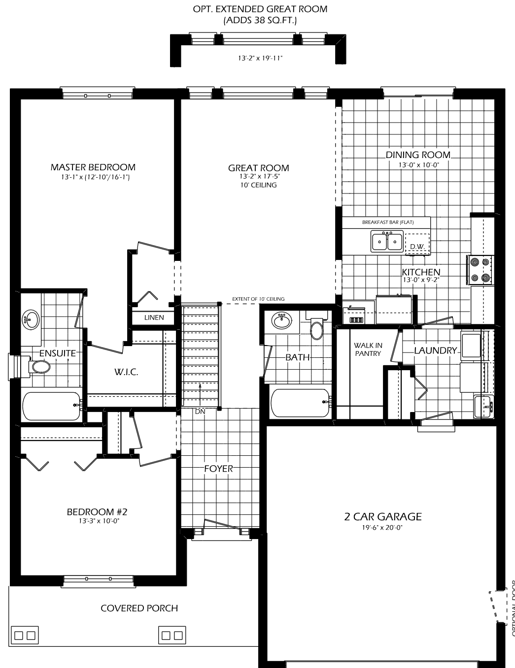
MAIN FLOOR 1460 SQ.FT. 8' CEILINGS (ON MAIN FLOOR)
