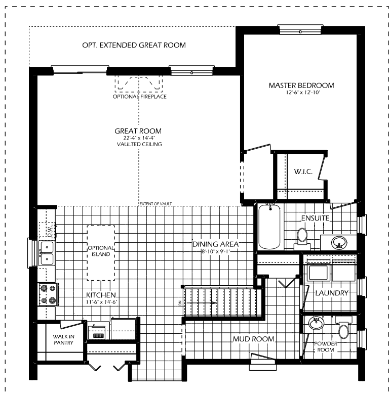
OPT. MAIN FLOOR WITH DINING AREA
