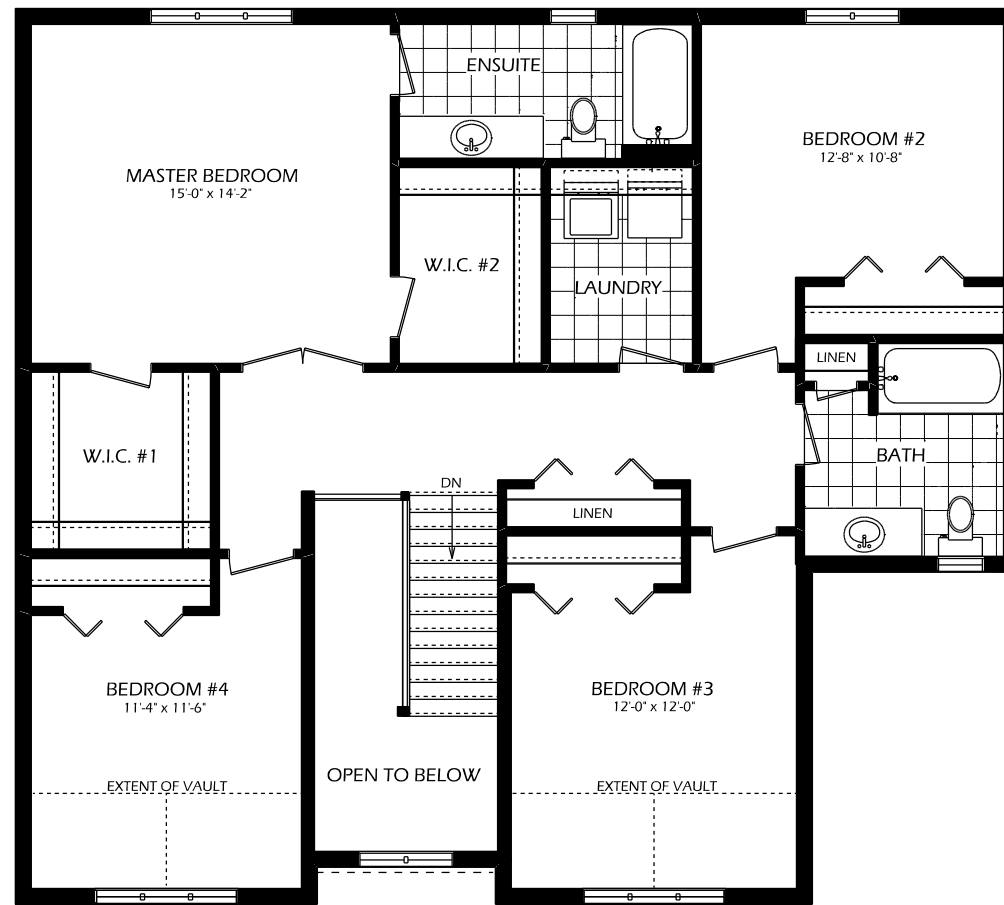
2ND FLOOR 1314 SQ.FT. 8' CEILINGS (2ND FLOOR)
