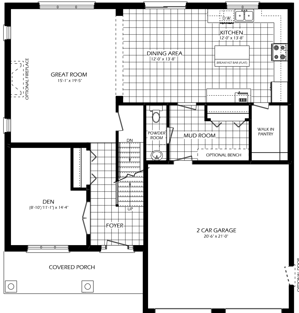
MAIN FLOOR 1238 SQ.FT. 8' CEILINGS (MAIN FLOOR)
